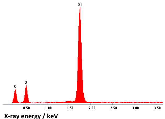
Example of EDX data showing spectra for a particle, likely to be silica.
